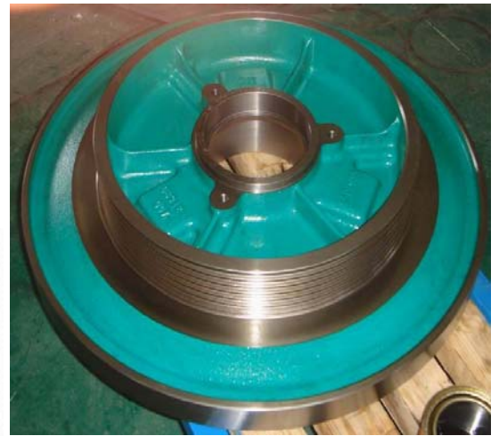
Tractive Wheel For Elevator (OD: 600~800mm)
