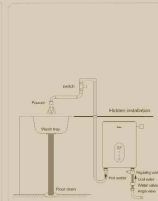
Installation diagram of Beke star
