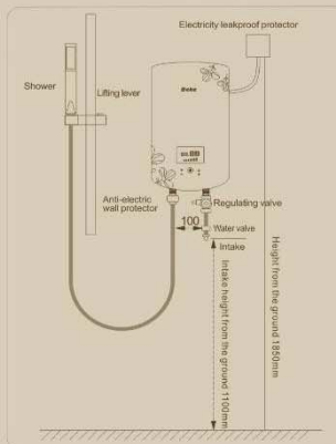
Installation diagram of water single supply
