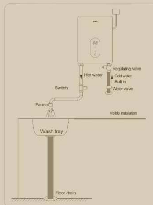
Installation diagram of Beke star
