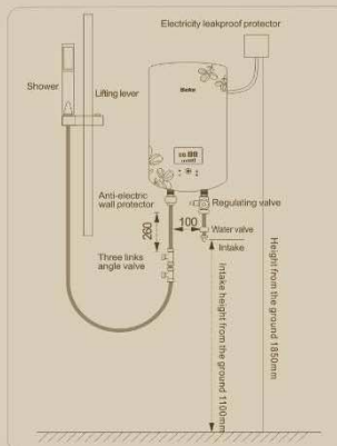
Installation diagram of water multiple supply
