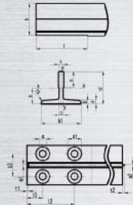
T型导轨加工图形 Drawings of Machined Guide Rail
