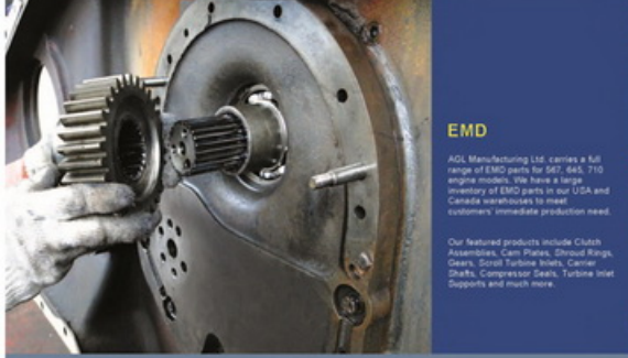
Clutch Assembly
